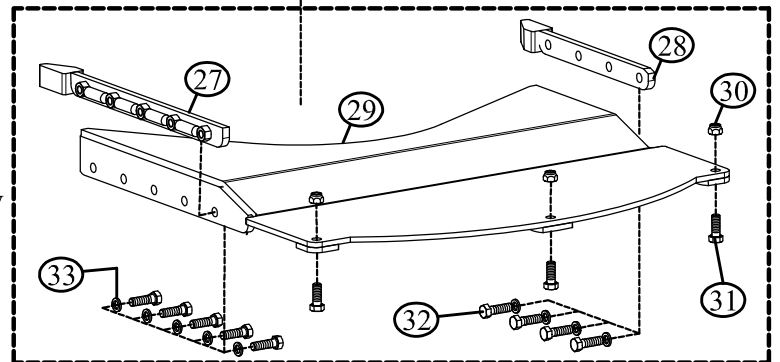
Option dessous la scie / Option under saw
